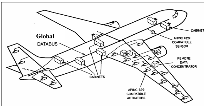
Fig. 16 Global bus based integrated avionics scheme for full aircraft configuration
