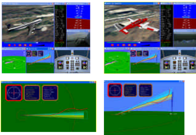
Fig. 10 NALVAS showing the configurable capability for different aircraft models with ILS operation
