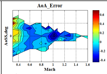
Figure 7. Beta-Mach envelope
